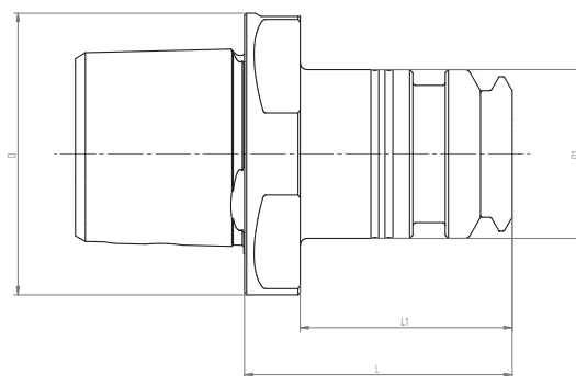
Dimensions/Dimensioni [mm]
